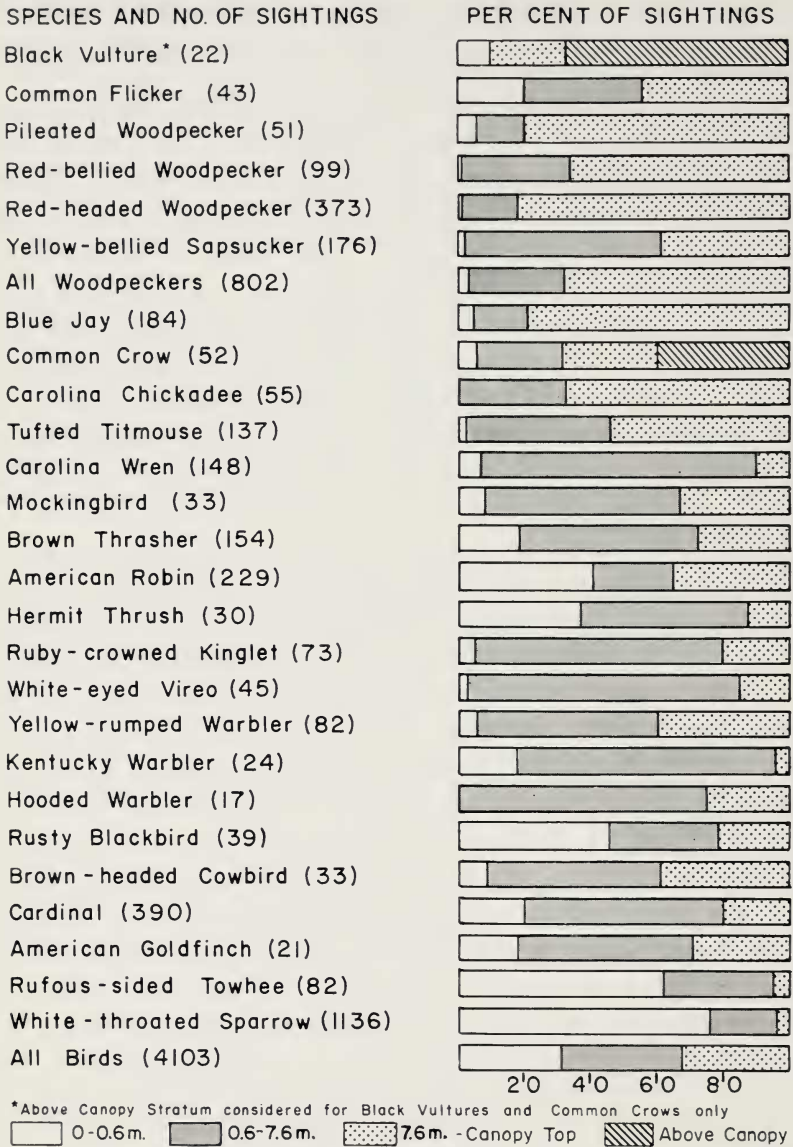
FIG. 1. Vertical height distributions of common birds.
